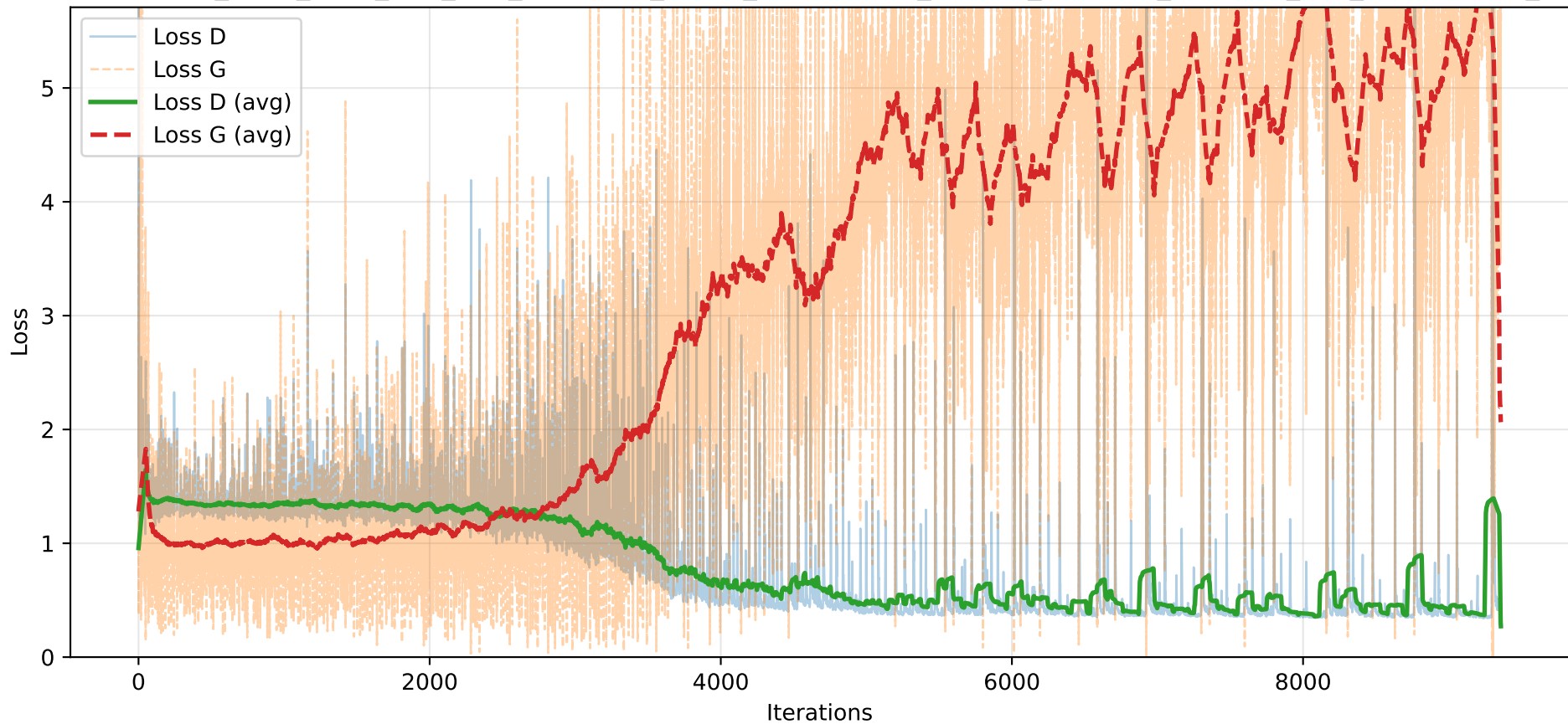
Losses - e20_b128_z100_kD1_kG1_Pbaseline_GAelu_DAl leakyrelu_Oadam_lrG0.002_lrD0.002_l0.9_be0.5-0.999_S42
