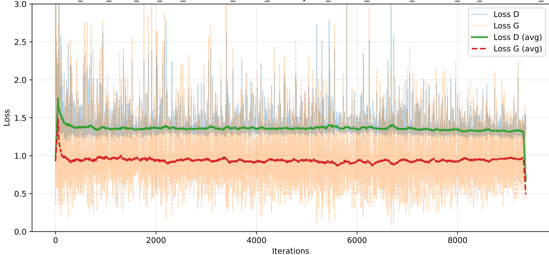
Losses - e20_b128_z100_kD1_kG1_Pbaseline_GAsilu_DAlaekyrelu_Oadam_lrG0.002_lrD0.002_l0.9_be0.5-0.999_S42
