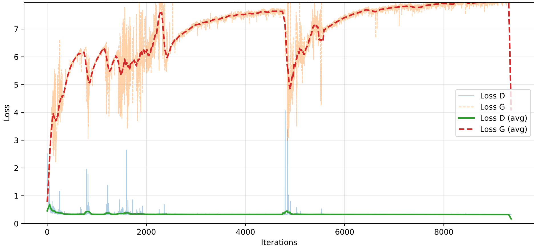
Losses - e20_b128_z100_kD2_kG1_PstrongerD_GArelu_DAlrelu_Oadam_lrG0.001_lrD0.002_l0.9_be0.5-0.999_S42
