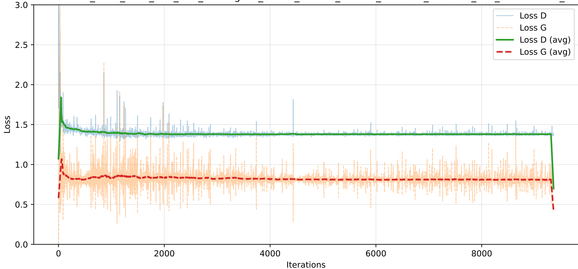
Losses - e20_b128_z100_kD1_kG2_PstrongerG_GAsilu_DAlrelu_Oadam_lrG0.002_lrD0.001_l0.9_be0.5-0.999_S42
