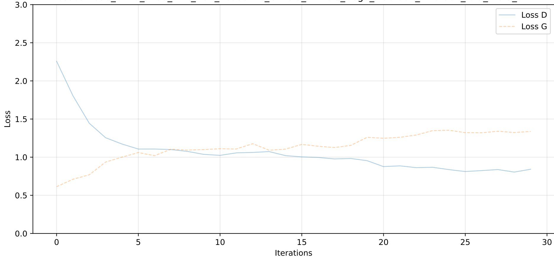
Losses - e30_b128_z100_kD1_kG1_Pbaseline_GArelu_DAlrelu_Osgd_lrG0.002_lrD0.002_l0.9_m0.5_S42
