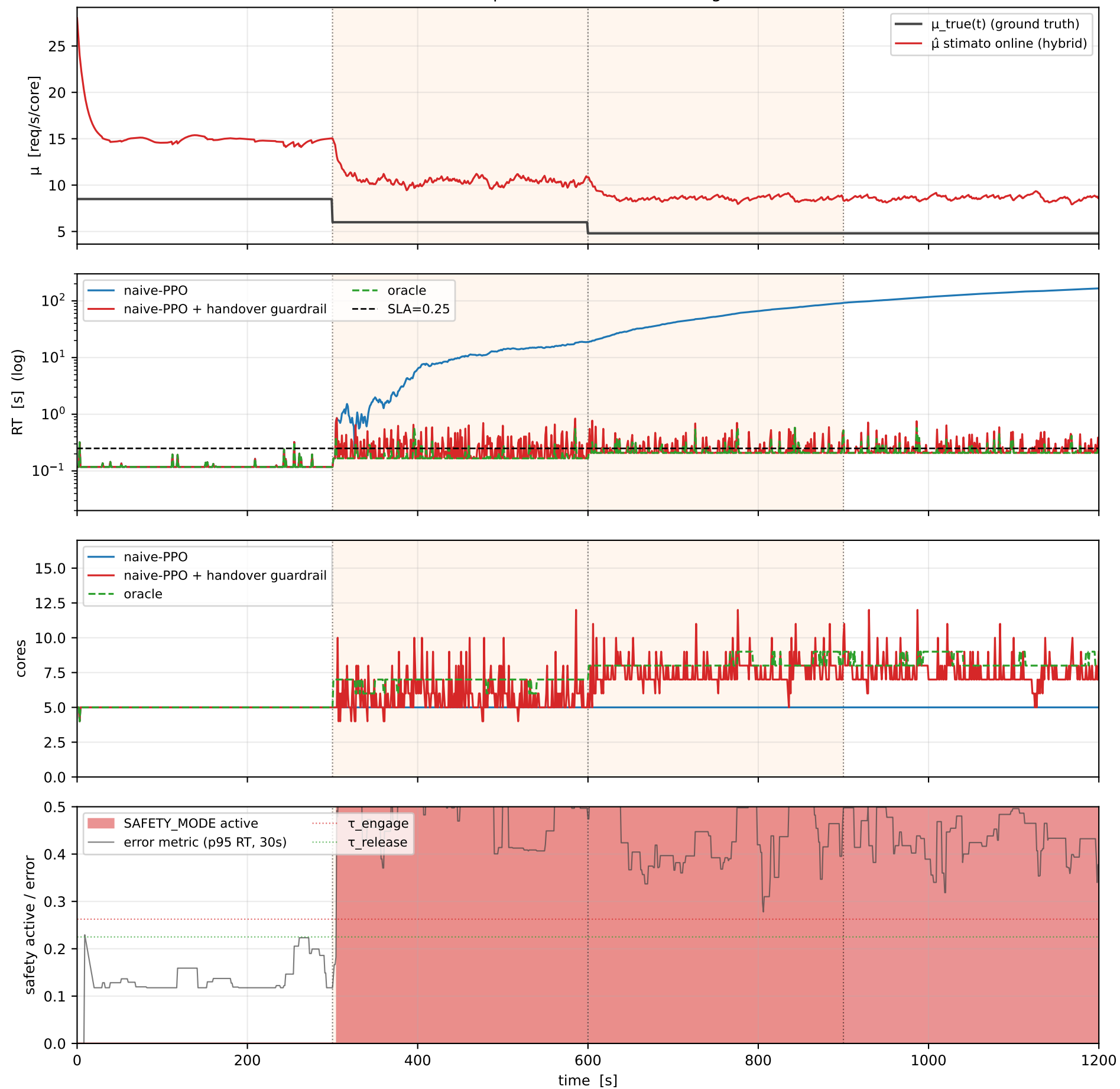
Mossa C — closed-loop in-vitro: PPO-naive vs +guardrail vs oracle
