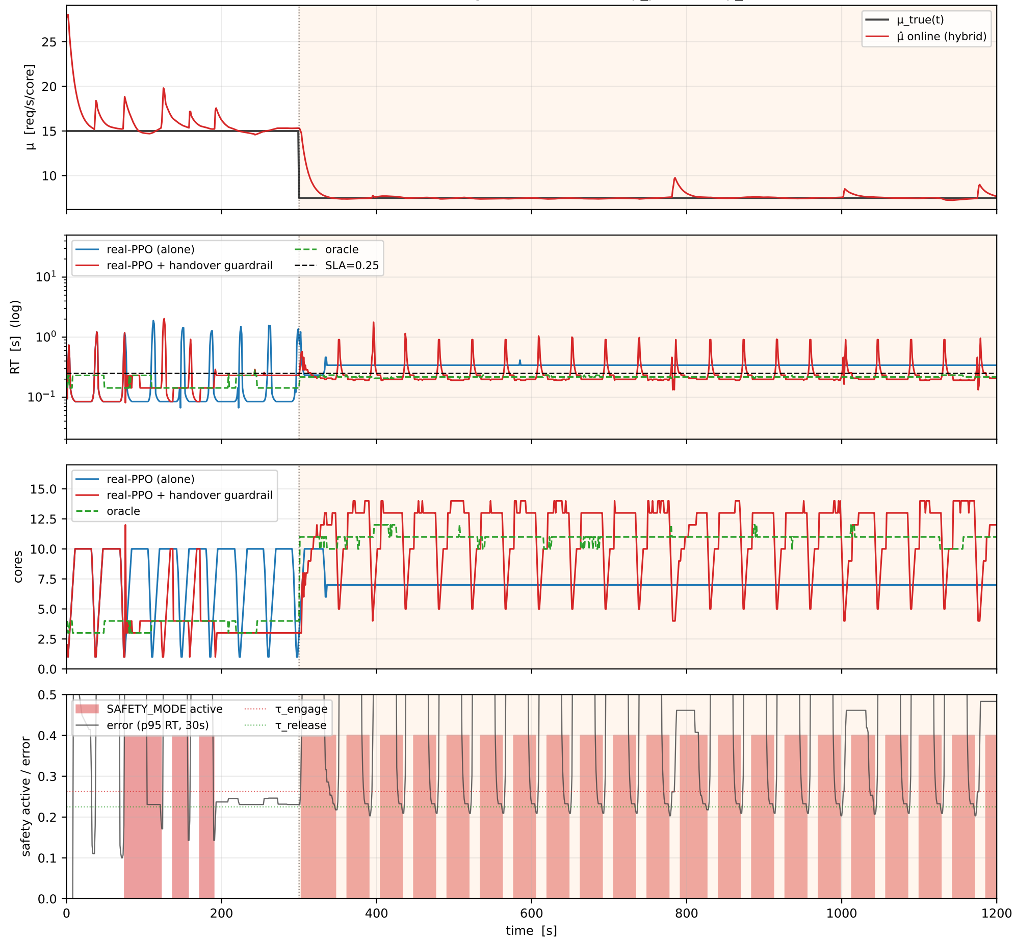
In-vitro REAL PPO + handover guardrail (calibrated: \mu_{\text{pre}}=15.0 , \mu_{\text{drift}}=7.5 )
