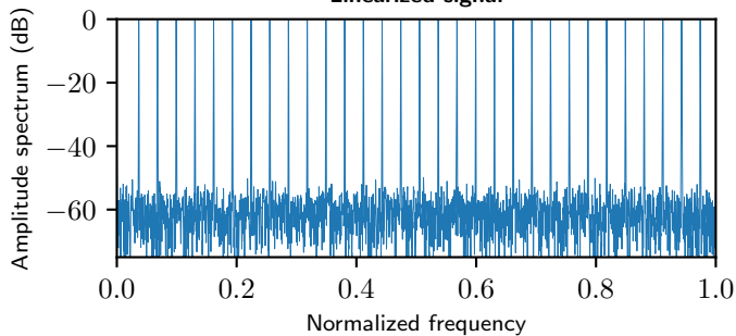
Linearized signal
