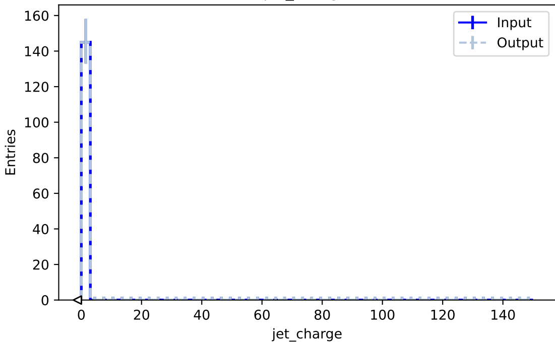
jet_charge
