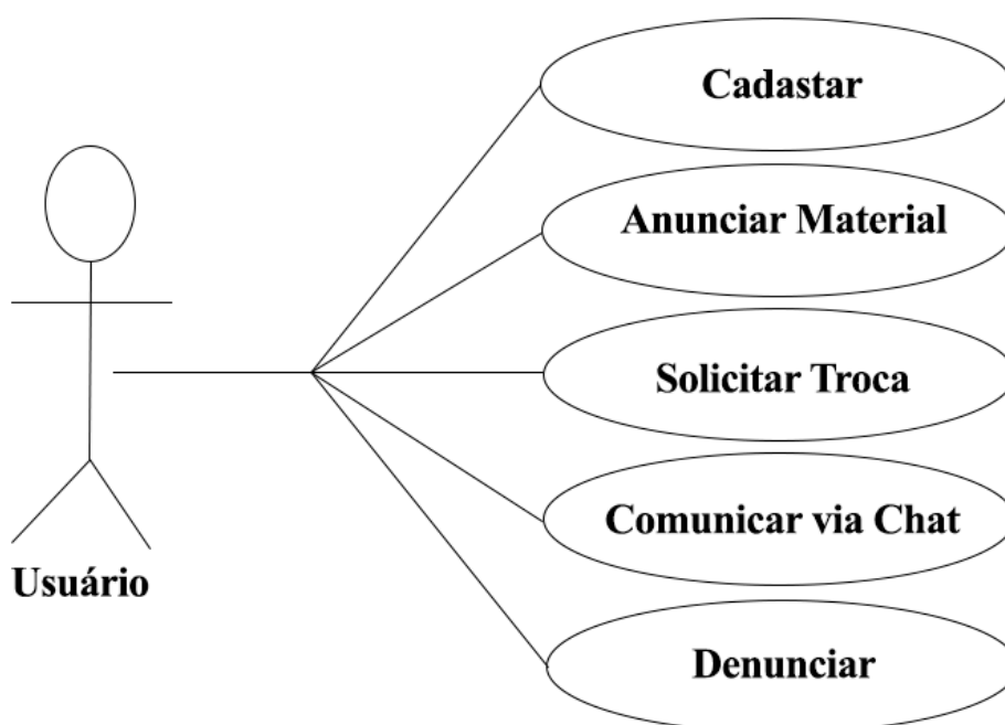
Figura 16: UML CIRCULARIS
