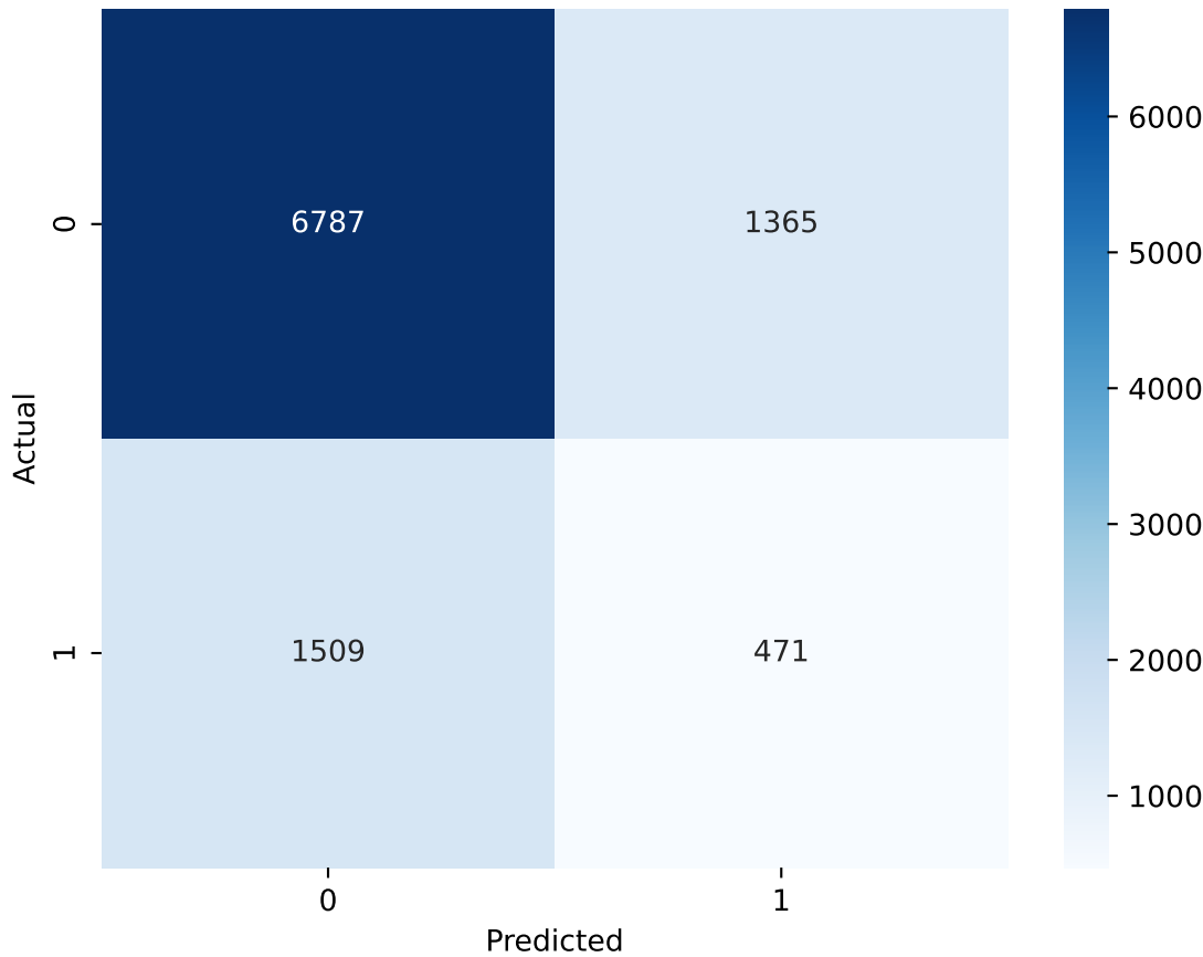
Logistic Regression
