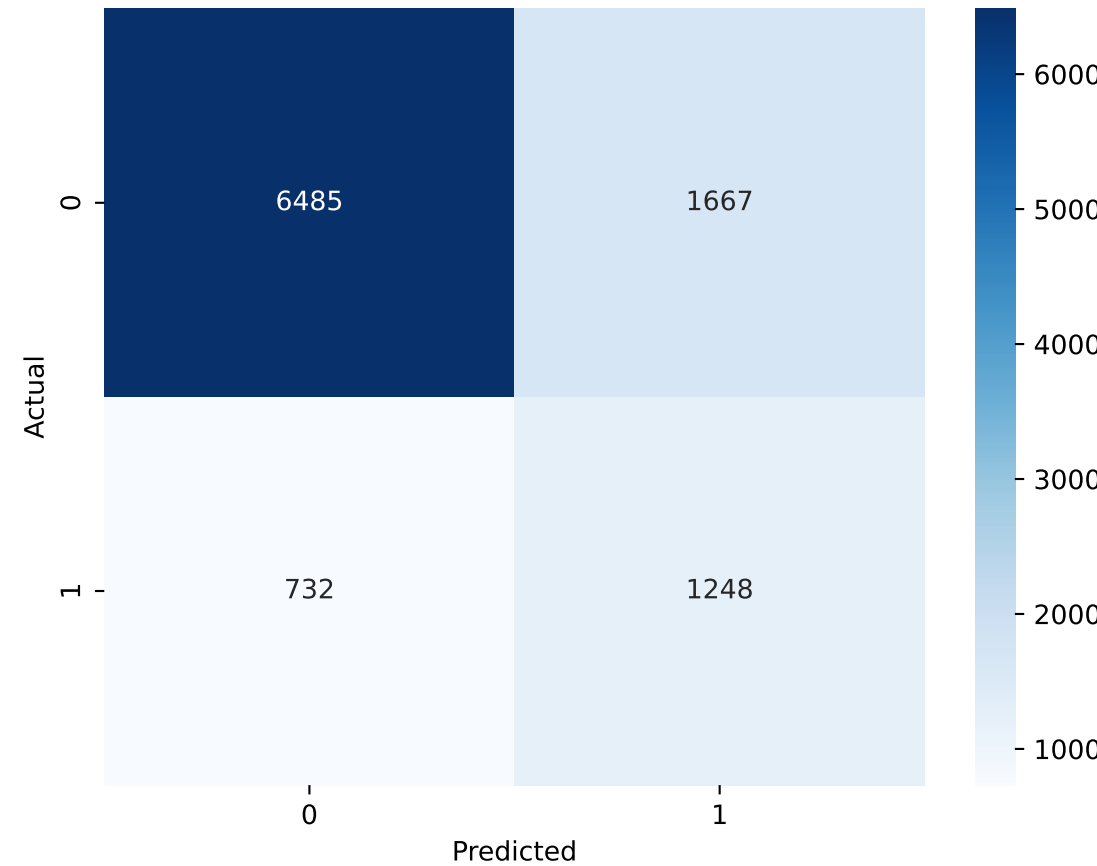
Decision Tree
