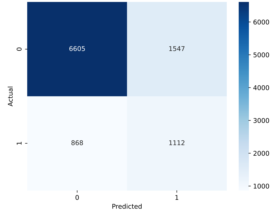
Neural Network
