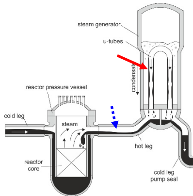
PWR safety injection
