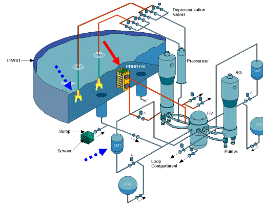
AP1000 passive safety system
