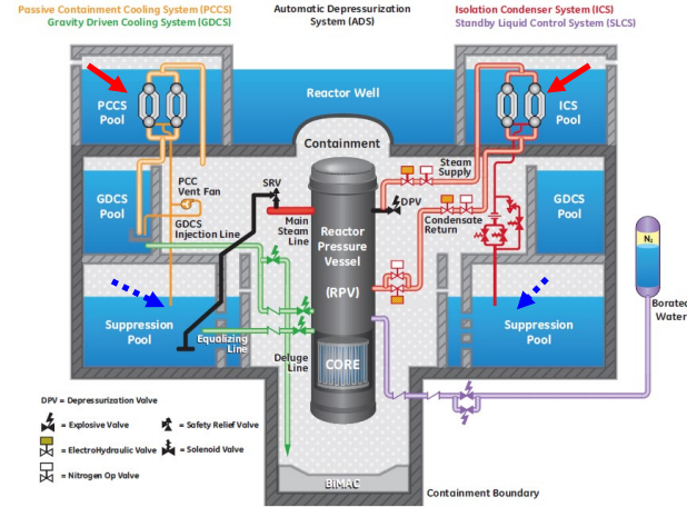
ESBWR passive safety system
