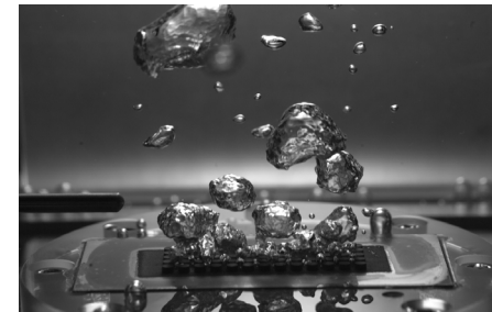
Pool Boiling
