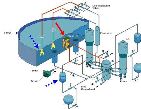
AP1000 passive safety system
