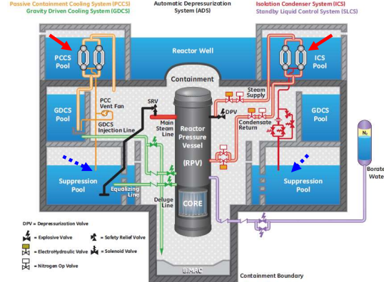
ESBWR passive safety system
