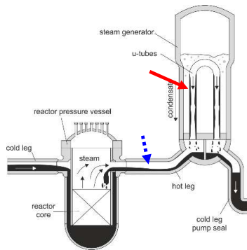
PWR safety injection
