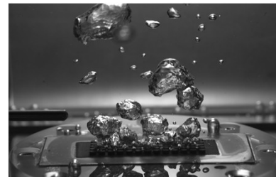
Pool Boiling
