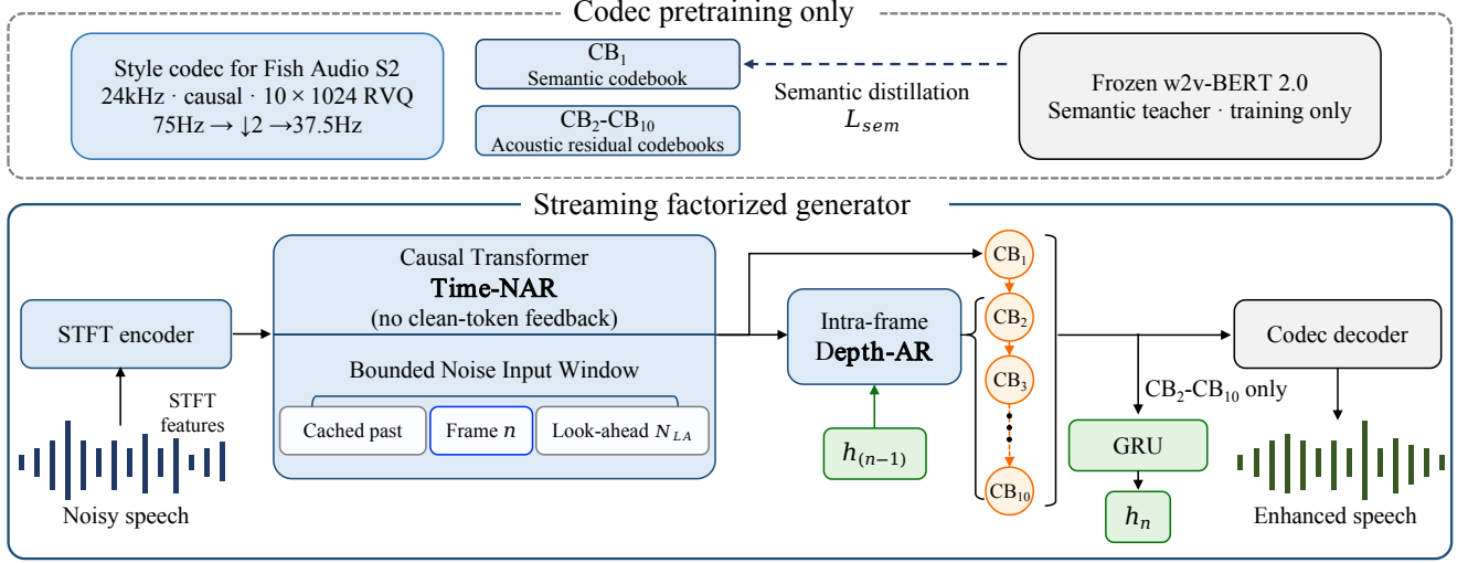
Fig. 1. Overview of FactorGSE. Codec pretraining distills w2v-BERT 2.0 semantics into CB_1 . At inference, time-NAR predicts CB_1 from bounded degraded-speech context without generated-token feedback; depth-AR then generates CB_2 – CB_{10} sequentially within each codec frame, while the GRU carries cross-frame acoustic history only through the residual branch.
