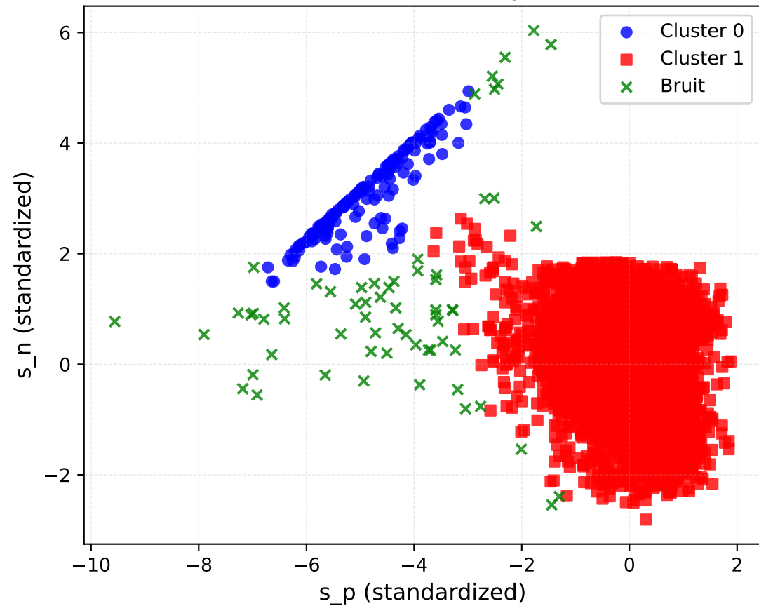
Clusters with noise points
