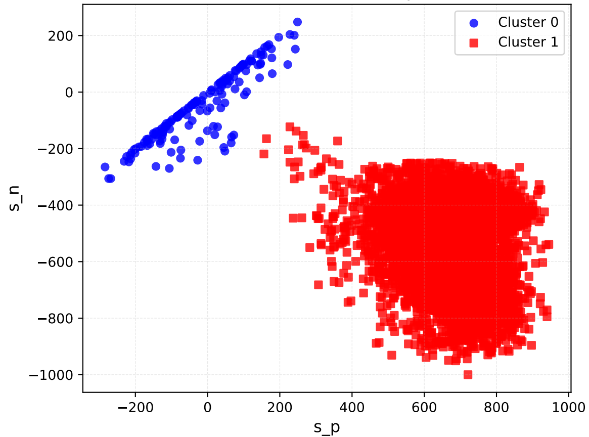
Clusters without noise points
