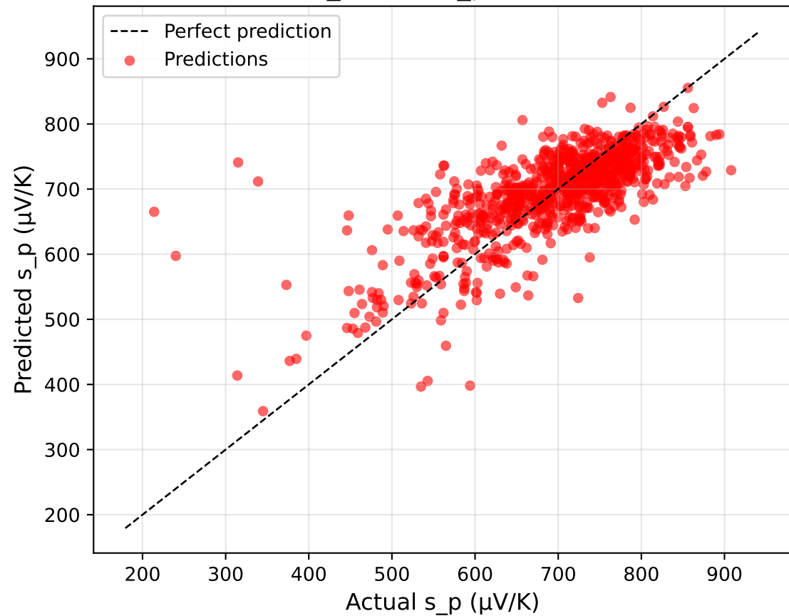
random_forest - s_p ( R^2 = 0.552 )
