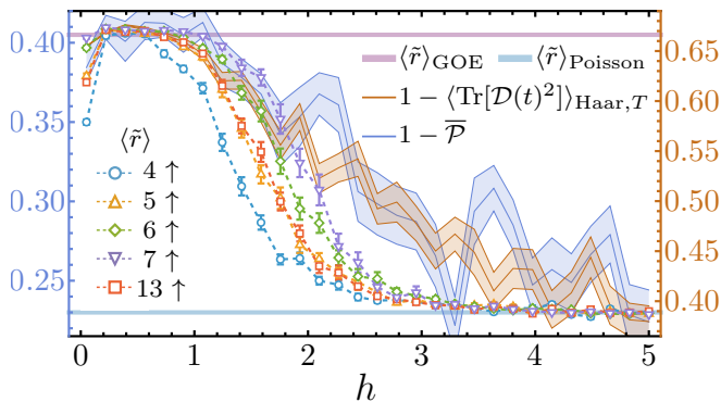
Figure 3. Comparison of spectral statistics and local single-spin dynamical probes for the Heisenberg model with random fields [Eq. (10)] as a function of disorder strength h . All quantities are averaged over 30 disorder realizations. Symbols: Mean level spacing ratio \langle \tilde{r} \rangle , computed for L = 18 within different magnetization sectors N_{\uparrow} (horizontal lines indicate GOE and Poisson limits). Solid lines: Local Single-spin dynamical probes computed for the spin at the first site ( L = 7 ), plotted as deviations from unity (impurities): Left axis (blue): averaged subsystem state impurity 1 - \overline{\mathcal{P}} [Eq. (6)] ( N = 50, T = 100 ); Right axis (brown): averaged Choi echo deviation 1 - \langle \text{Tr}[\mathcal{D}(t)^2] \rangle_{\text{Haar}, T} [Eq. (8)] ( T = 100 ). Shaded bands and error bars indicate the standard deviation.
