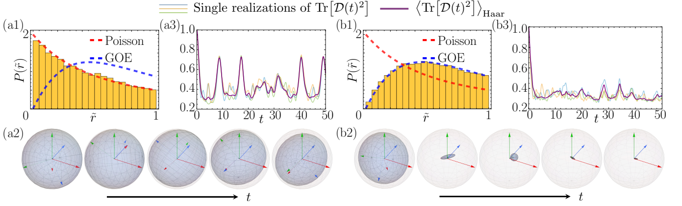
Figure 1. Spectral and single-spin dynamical behavior in regular and chaotic regimes of the mixed-field Ising model [Eq. (9)]. Panel (a) corresponds to an integrable regular regime [(h_z, J) = (1.446, 0.05)] and the chaotic panel (b) to a chaotic regime [(h_z, J) = (0.48, 0.8)] , with fixed h_x = 1 . (a1) , (b1) Distribution of nearest-neighbor level spacing ratios P(\tilde{r}) for L = 16 (even sector), compared to Poisson (red dashed) and GOE (blue dashed) predictions. (a2) , (b2) Action of the quantum channel \mathcal{E}_t on the Bloch sphere of the probe spin ( L = 7 ). The solid arrows represent the initial Cartesian axes of the Bloch sphere ( x, y, z ), while the dotted arrows indicate their transformed orientation at later times. In the chaotic regime , the quantum channel induces a rapid contraction of the sphere volume, contrasting with the coherent precession in the regular case. (a3) , (b3) Time evolution of the Choi echo \text{Tr}[\mathcal{D}(t)^2] ( L = 7 ). Low-opacity lines represent single realizations with random initial product states of the environment; the thick purple line corresponds to the analytical Haar-averaged Choi echo \mathbb{E}[\text{Tr}[\mathcal{D}^2(t)]] derived in Eq. (7).
