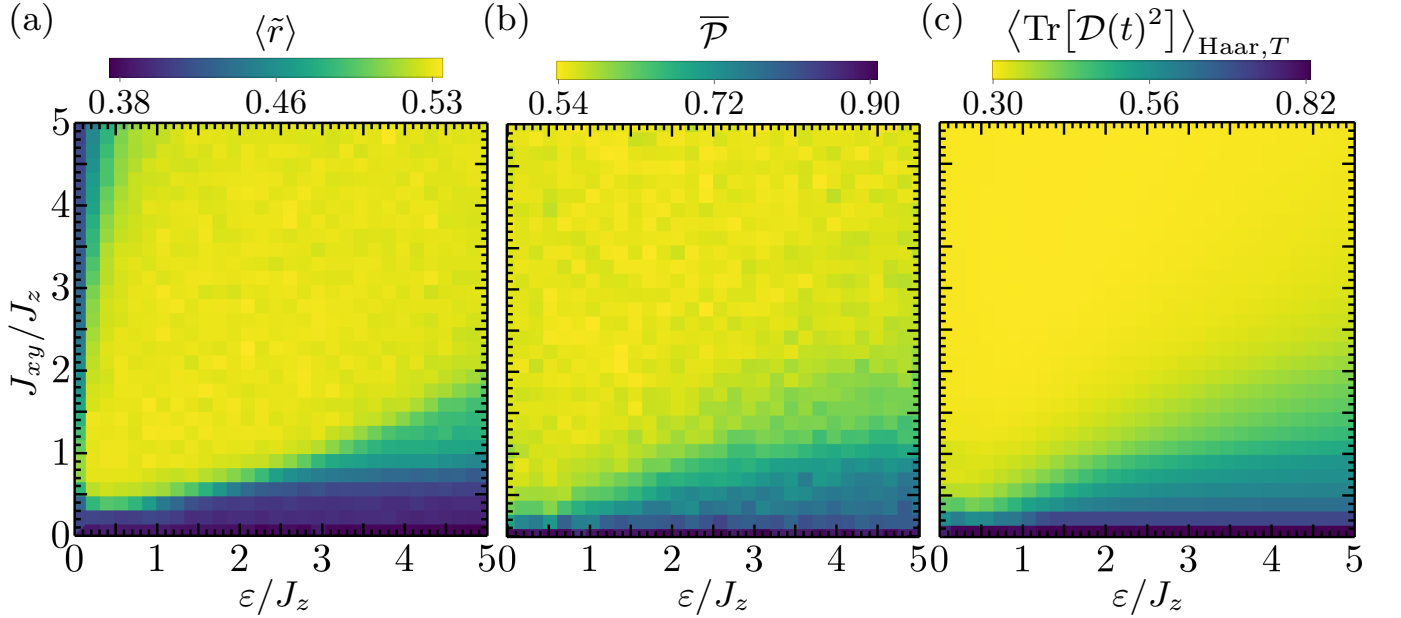
Figure 4. Comparison of spectral statistics and local single-spin dynamical probes for the XXZ model with a local defect [Eq. (11)] as a function of J_{xy}/J_z and \varepsilon/J_z . (a) Mean level spacing ratio \langle \tilde{r} \rangle , computed for L = 18 ( N_\uparrow = 7 ) with the defect at site d = 9 . (b), (c) Local Single-spin dynamical probes computed for the spin at the first site ( L = 7 ) with the defect at site d = 3 : (b) averaged subsystem state purity \overline{\mathcal{P}} [Eq. (6)] ( N = 50 , T = 100 ); (c) averaged Choi echo \langle \text{Tr}[\mathcal{D}(t)^2] \rangle_{\text{Haar}, T} [Eq. (8)] ( T = 100 ). In both configurations, the defect placement explicitly breaks spatial reflection symmetry.
