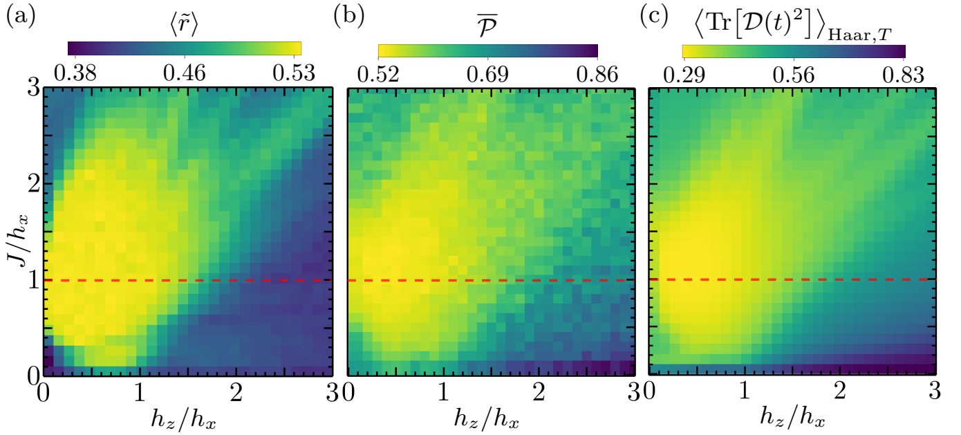
Figure 2. Comparison of short-range spectral statistics and local single-spin dynamical probes for the mixed-field Ising model [Eq. (9)] as a function of h_z/h_x and J/h_x . (a) Mean level spacing ratio \langle \tilde{r} \rangle , computed for L = 16 within the even symmetric sector. (b), (c) Local Single-spin dynamical probes computed for the spin at the first site ( L = 7 ): (b) averaged subsystem state purity \overline{\mathcal{P}} [Eq. (6)] ( N = 50 , T = 100 ); (c) averaged Choi echo \langle \text{Tr}[\mathcal{D}(t)^2] \rangle_{\text{Haar}, T} [Eq. (8)] ( T = 100 ). The horizontal red dashed line ( J/h_x = 1 ) indicates the parameter cut where the correspondence between \langle \tilde{r} \rangle and \overline{\mathcal{P}} was analyzed in Ref. [17] for h_z/h_x \in [0, 2.5] .
