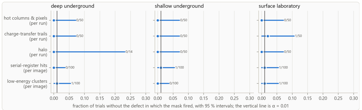
Clopper–Pearson 95 % intervals; the vertical line is \alpha = 0.01 . Intervals are wide because 50 runs cannot resolve 0.01 from 0.03.
