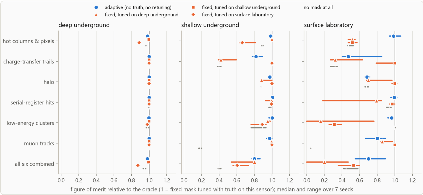
Figure of merit relative to the oracle tuned with truth on the same sensor (vertical line). Markers are medians over 7 seeds, whiskers the range. The deep-underground sensor has few target events, so every version sits near 1 there.
