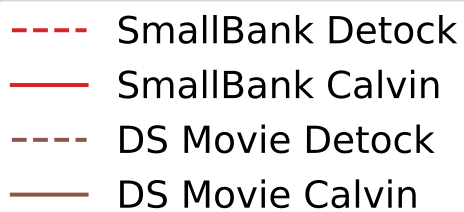
Throughput
