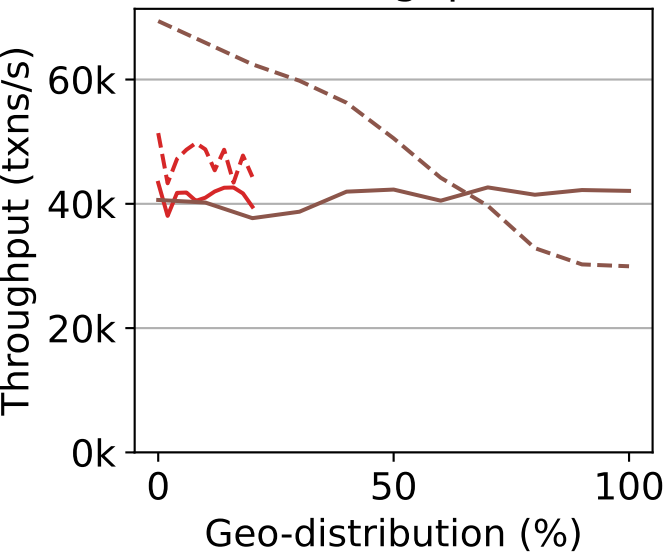
Throughput
