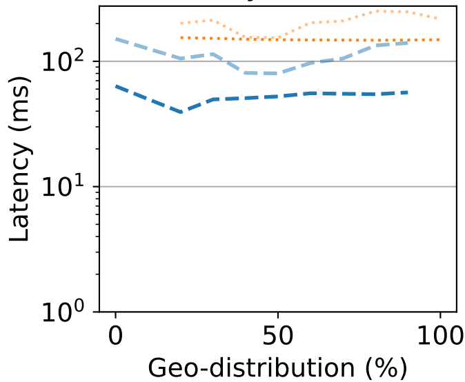
Latency Ablations
