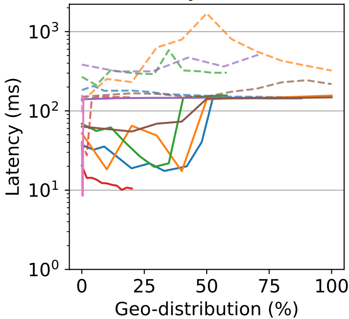
Latency (Detock)
