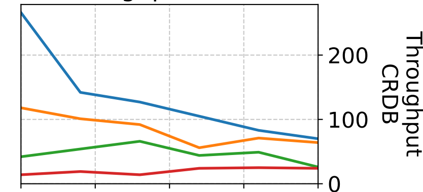
Throughput (CRDB)
