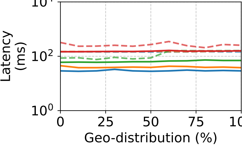
Latency (Calvin)
