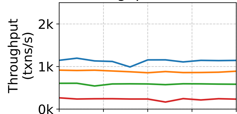
Throughput (Calvin)
