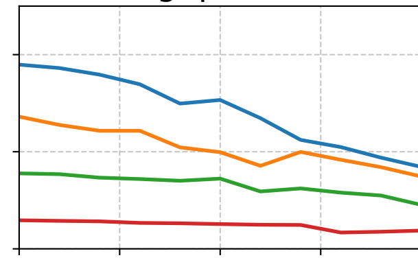
Throughput (SLOG)
