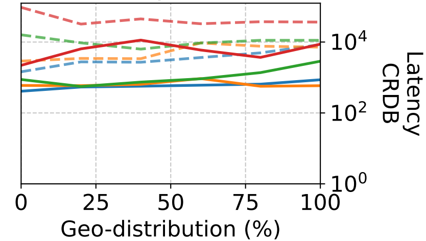
Latency (CRDB)
