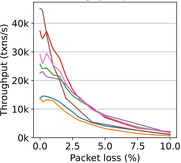
Throughput (Janus)
