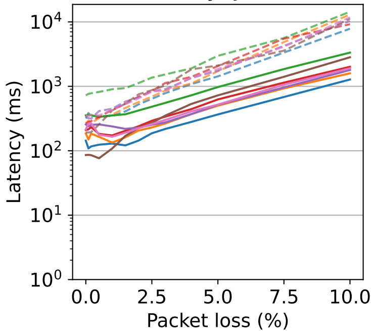
Latency (Janus)
