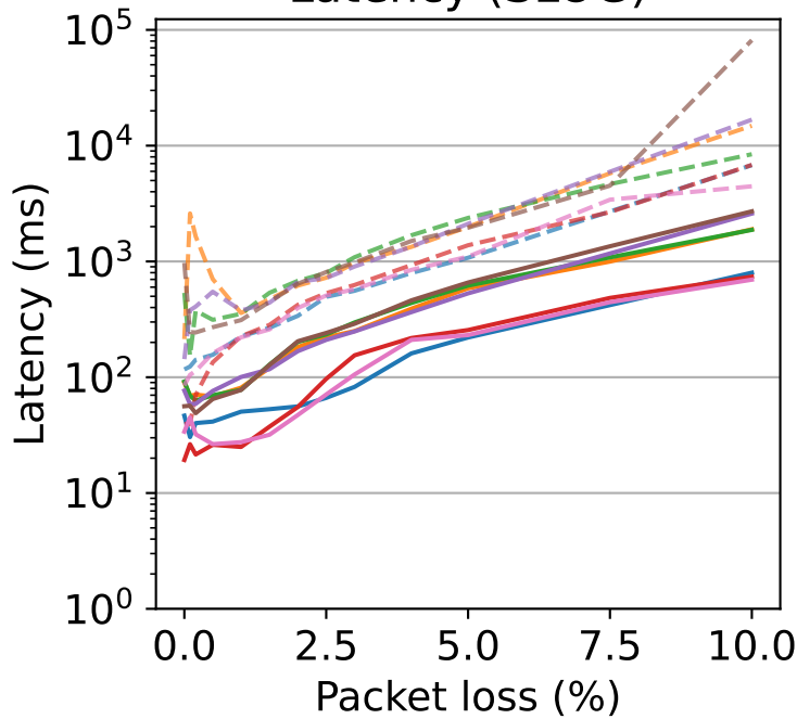
Latency (SLOG)
