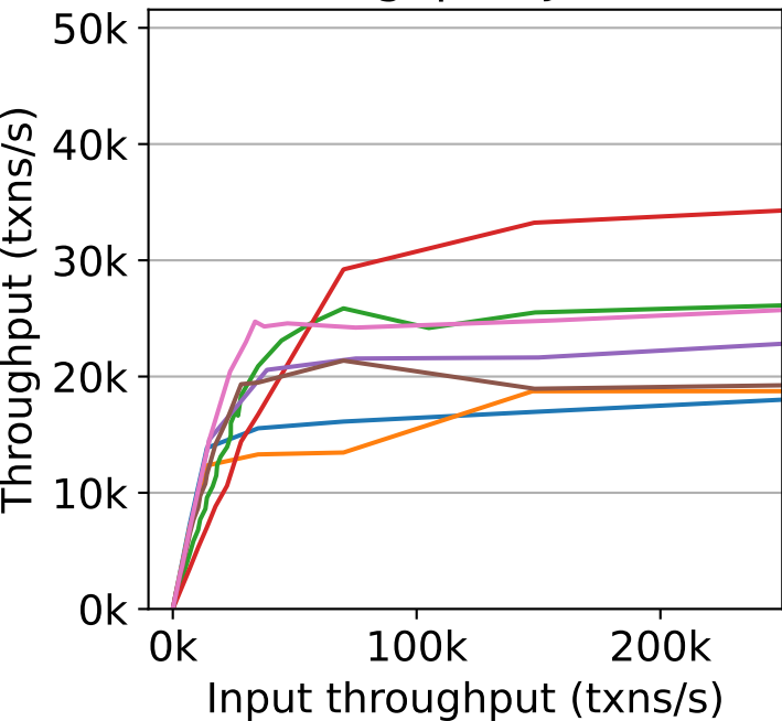
Throughput (Janus)
