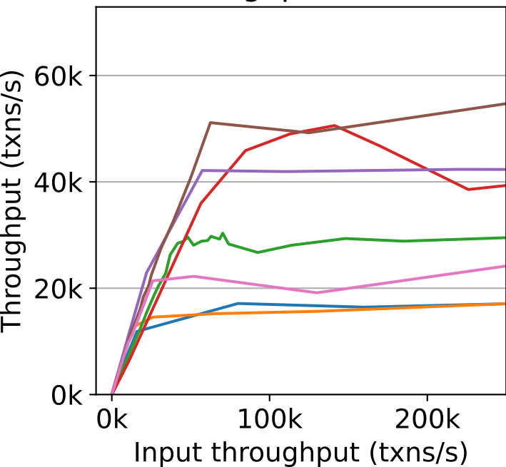
Throughput (SLOG)
