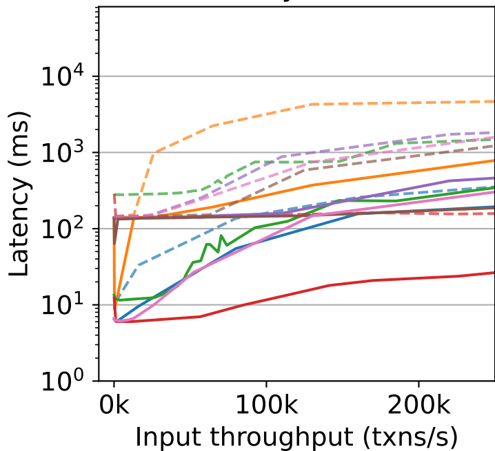
Latency (SLOG)
