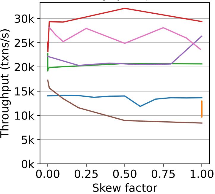
Throughput (Janus)
