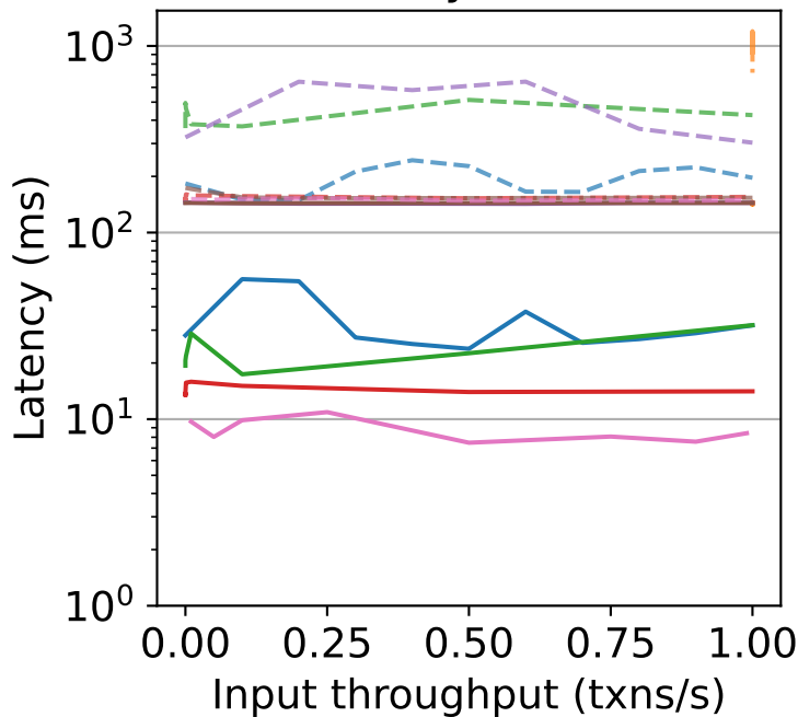
Latency (SLOG)
