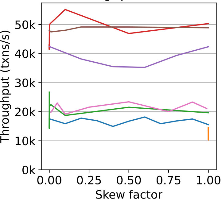
Throughput (SLOG)
