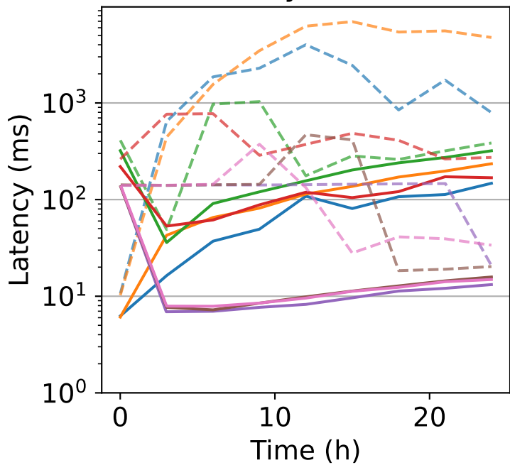
Latency (Calvin)
