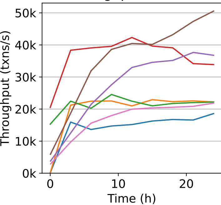
Throughput (Calvin)
