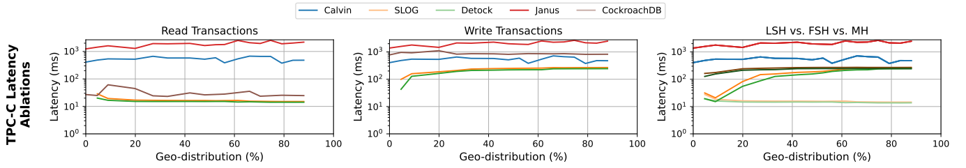
Fig. 12. The TPC-C read vs. write and LSH vs. FSH vs. MH latency ablations under the access patterns scenario. In the LSH vs. FSH vs. MH subplot the lightest shades represent LSH, medium shades represent FSH and darkest shades represent MH transactions.
