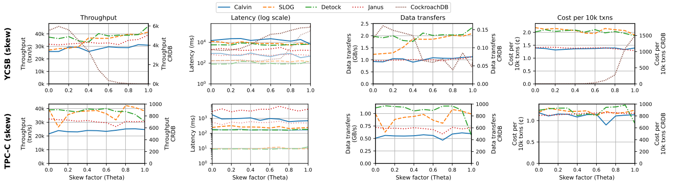
Fig. 14. The YCSB and TPC-C throughput, latency, data transfers, and cost per transaction under access skew. Opaque lines in the latency figure represent p50 and bold ones p99.
