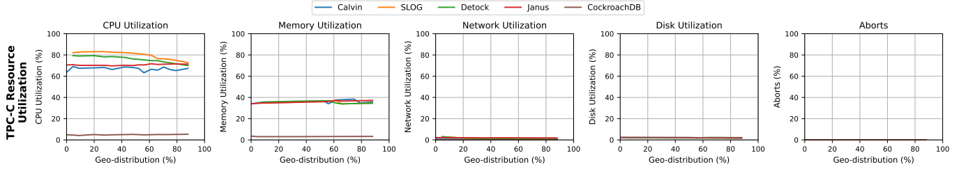
Fig. 13. The TPC-C CPU, memory, network, and disk utilization, and abort rate under the access patterns scenario.
