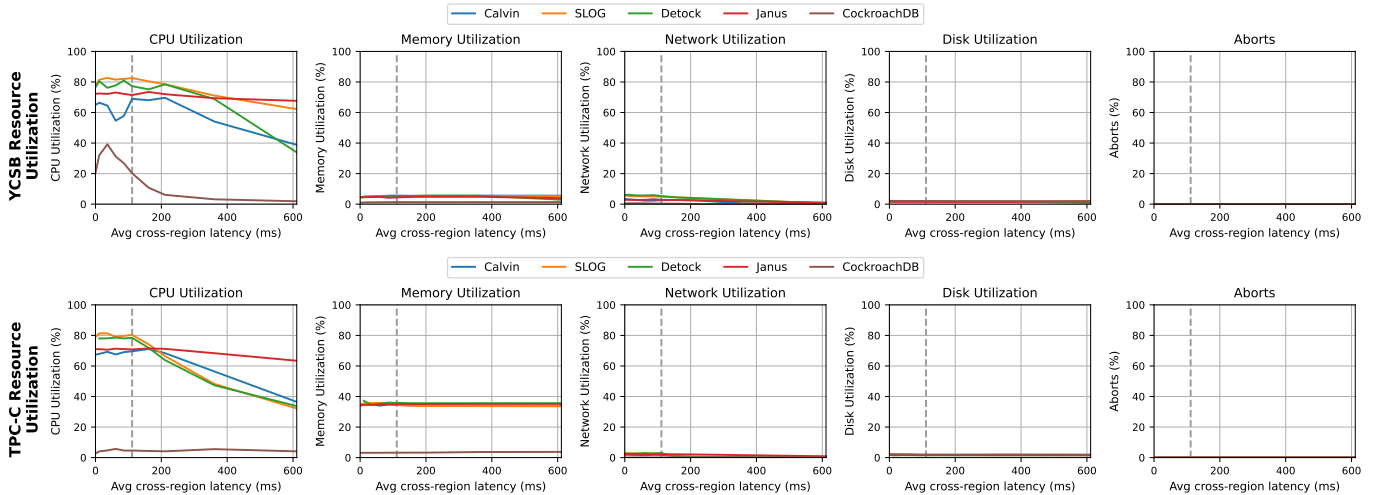
Fig. 15. The YCSB and TPC-C CPU, memory, network, and disk utilization, and abort rate under extra network latency and jitter. The dashed vertical line represents the average cross-region latency in the default geo-distribution setup.
