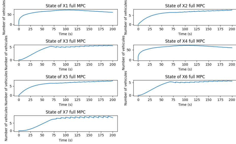
Figure 4: MPC cells states
