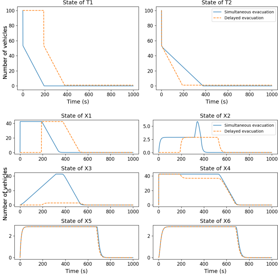
Figure 2: Two different evacuation strategies : simultaneous or delayed evacuation
