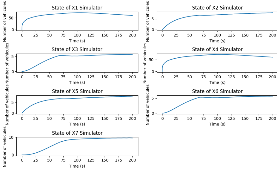
Figure 5: Simulator cells states
