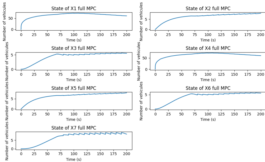
Figure 3: MPC and simulator tank states
