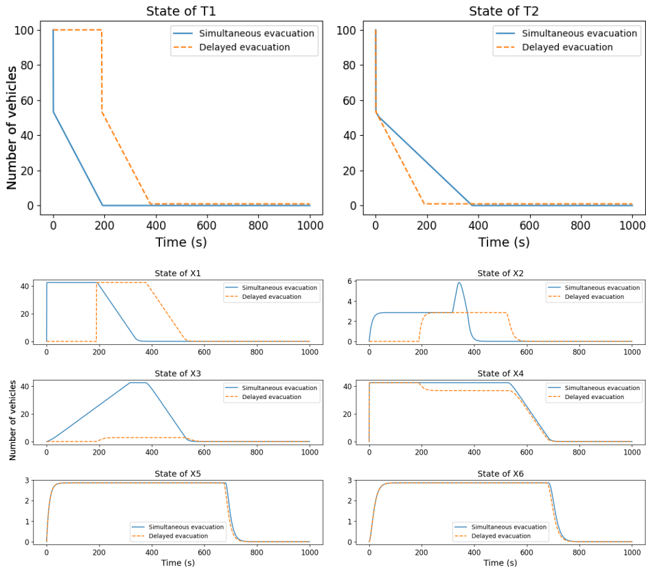
Figure 2: Two different evacuation strategies : simultaneous or delayed evacuation
