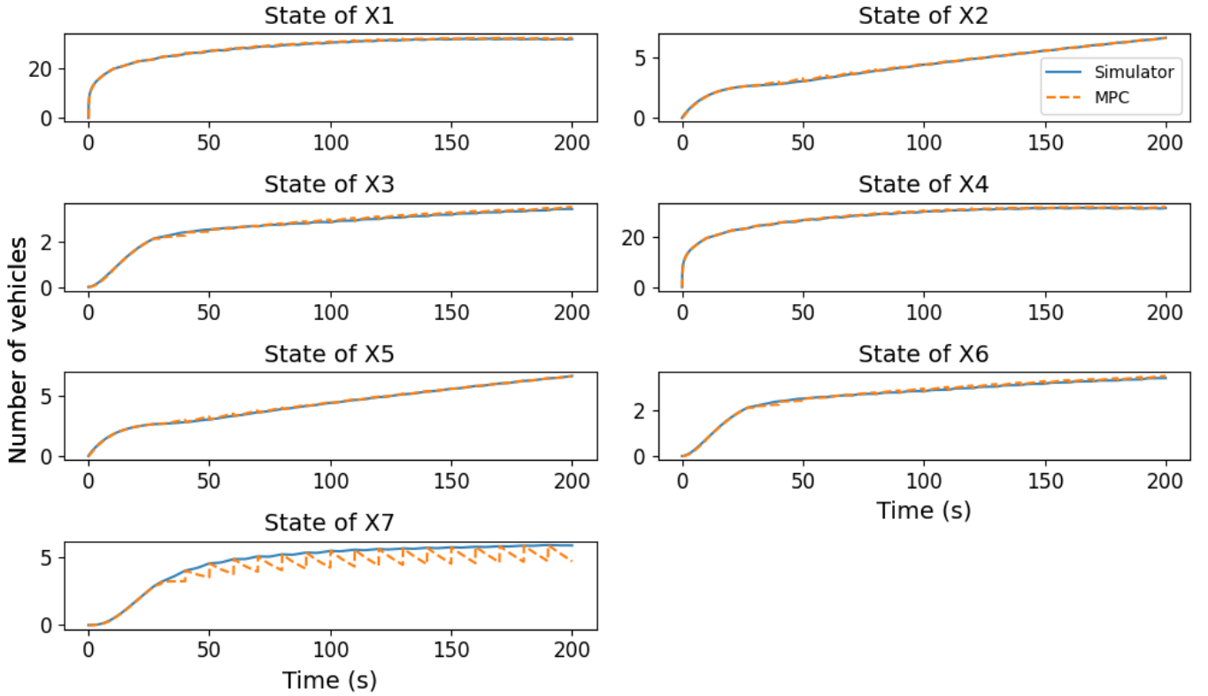
Figure 9: MPC cells states
