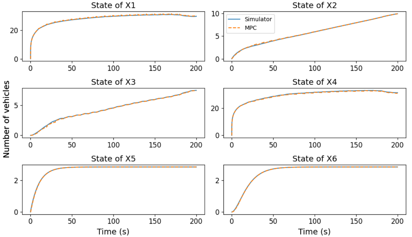
Figure 7: MPC cells states
