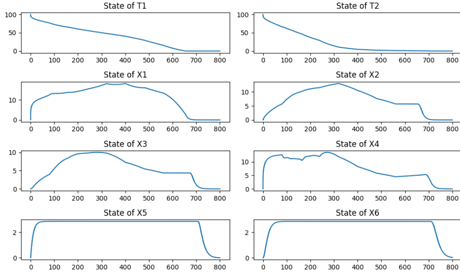
Figure 5: MPC solution for the line graph with a horizon of 1600 steps
