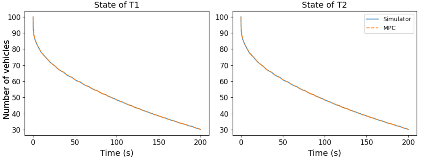
Figure 8: MPC tank states
