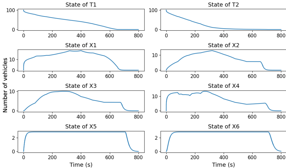
Figure 6: MPC solution for the line graph with a horizon of 1600 steps
