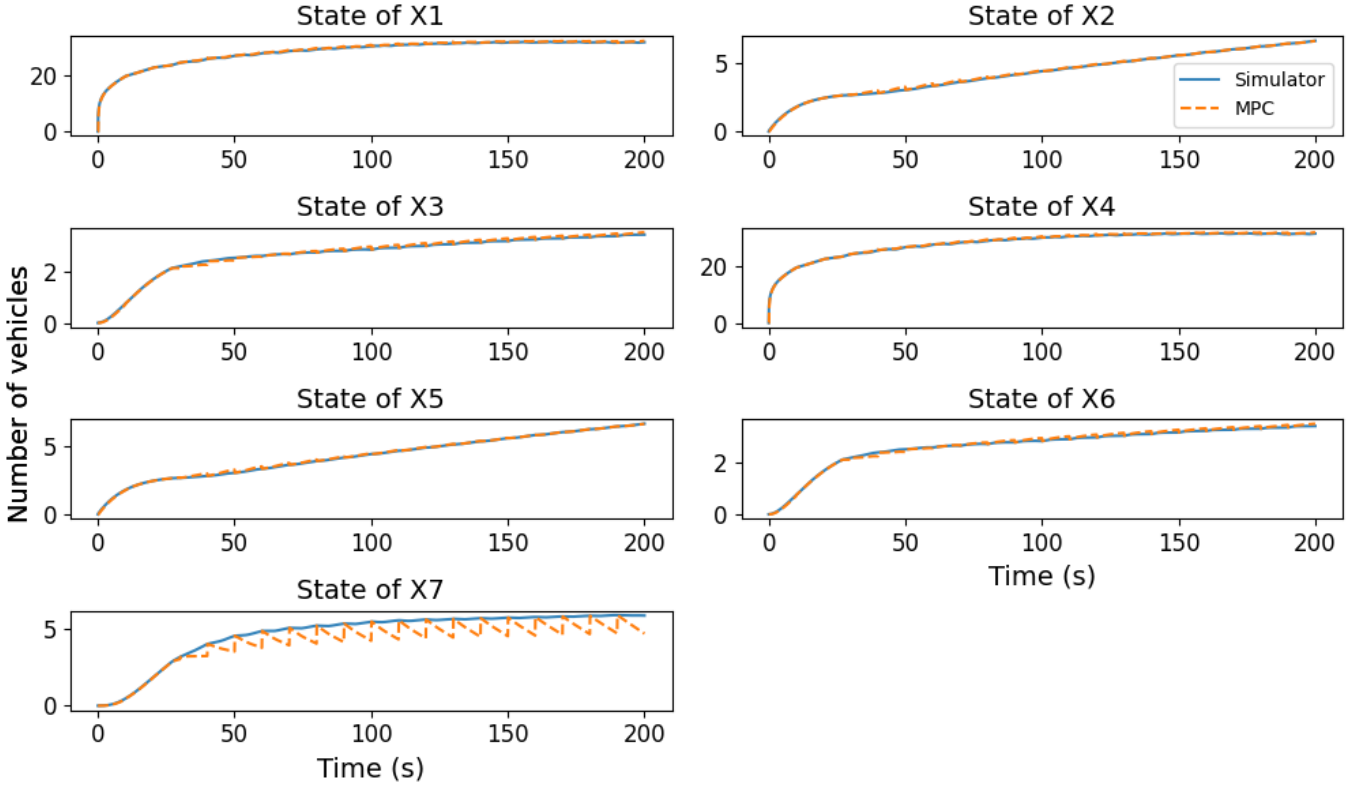
Figure 8: MPC cells states
