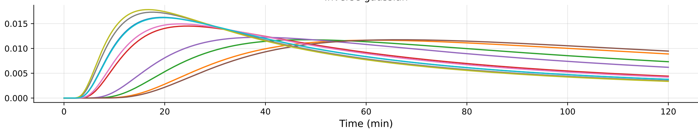
Inverse gaussian
