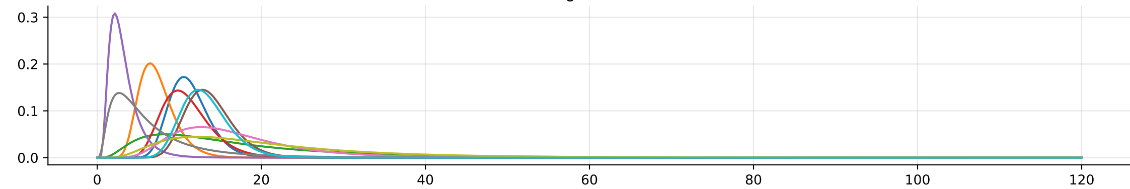
Weibull
