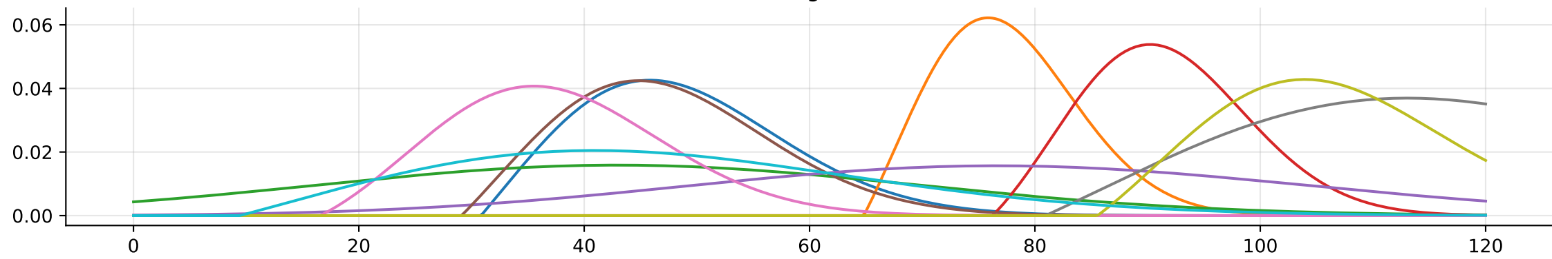
Biexponential
