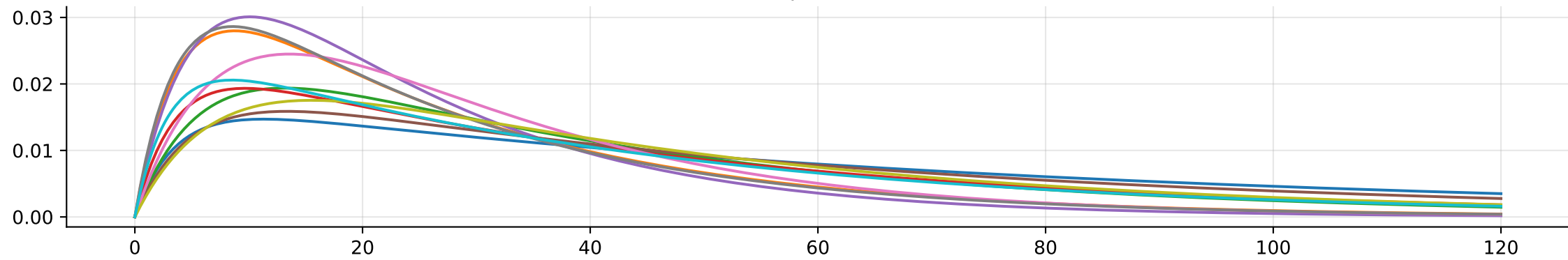
Gamma
