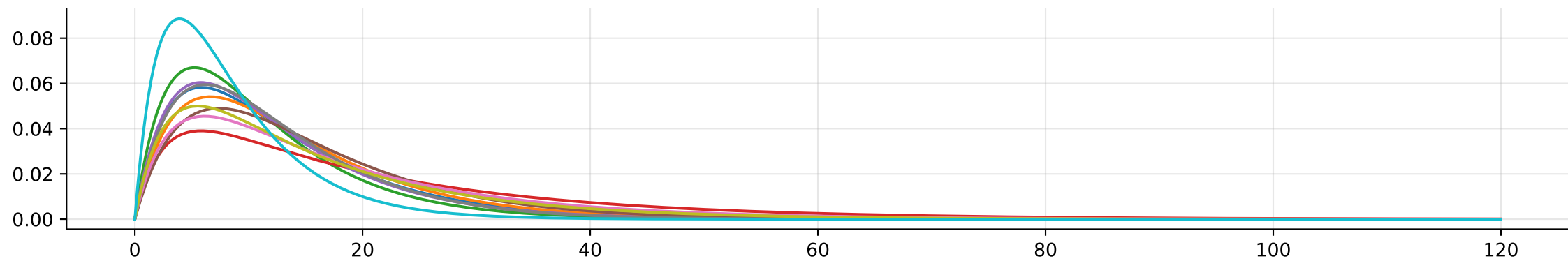
Inverse gaussian
