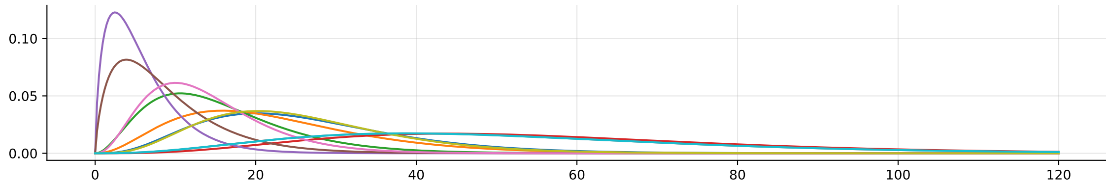
Lognormal
