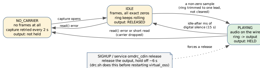
Figure 7.2: The daemon's state machine. The output device is held only in PLAYING; the capture device is held for the whole session.
