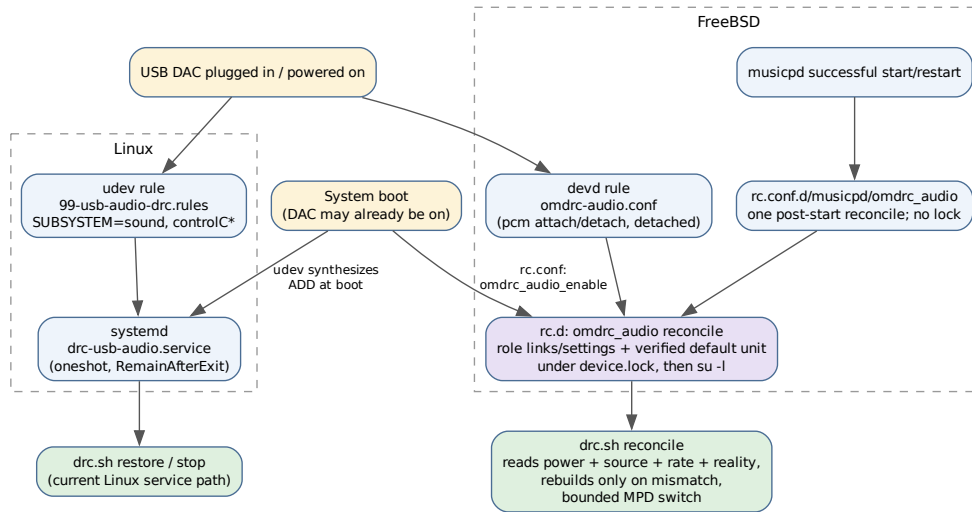
Figure 3.1: Linux’s current udev/systemd edge and the redesigned FreeBSD devd/rc.d level reconciliation.
