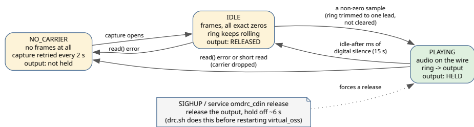
The daemon’s state machine. The output device is held only in PLAYING; the capture device is held for the whole session.
