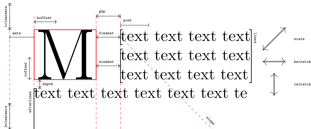
Figure 1: Anatomy of the initial package options; note that, for clarity, options scale , hstretch , and vstretch are visually displaced to the side, which are options that directly operate on the initial object in the red bounded box.
