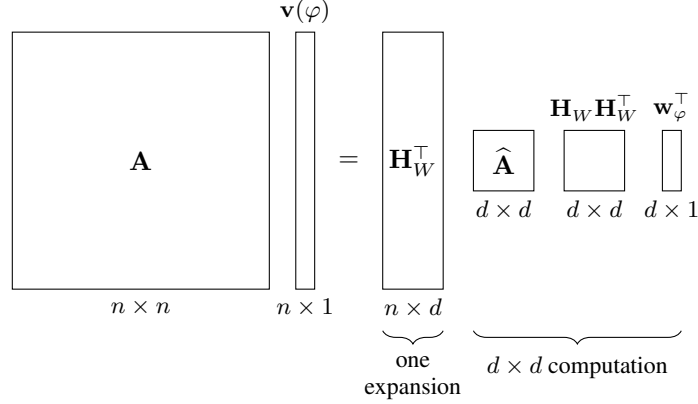
Figure 6: The compressed modal accumulation of (3), \mathbf{A} \mathbf{v}(\varphi) = \mathbf{H}_W^T \hat{\mathbf{A}} (\mathbf{H}_W \mathbf{H}_W^T) \mathbf{w}_\varphi^T , with d \ll n . To the right of \mathbf{H}_W^T , every block is d \times d or d \times 1 , so the accumulation is a d \times d computation, and one expansion through \mathbf{H}_W^T ; the threshold checks of (1) then apply to the expanded vector unchanged. The \mathbf{H}_W \mathbf{H}_W^T is as a single d \times d block, because it is formed once from the geometry and shared across propositions \varphi .
