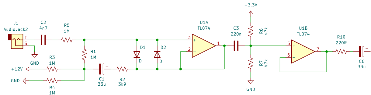
Bootstrapped Piezo Pre-amp
