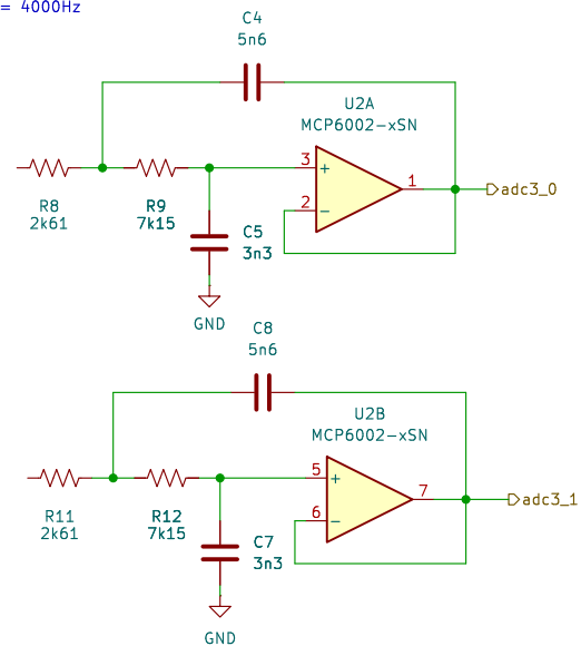
Sallen-Key 2nd Order Low-Pass F c = 4000Hz
