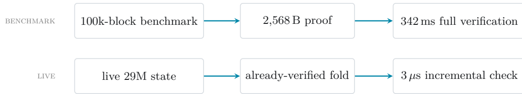
Figure 5: Fold verification flow — two lanes, two measurements. The 342 ms full verification was measured at the 100k-block benchmark; the 3\mu\text{s} incremental check runs on the live 29M-block network against an already-verified fold state. The lanes are separate experiments and must not be read as one pipeline; full verification of the live 29M fold has not yet been separately benchmarked.
