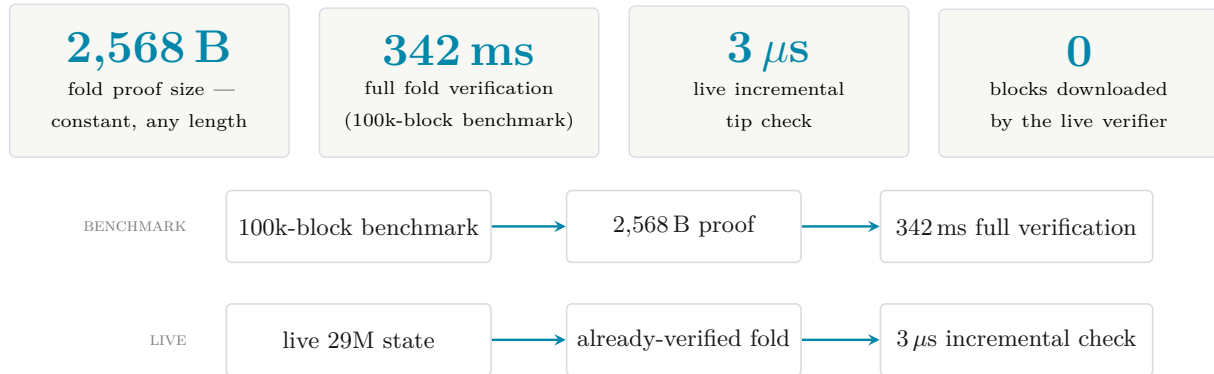
Figure 5: Fold verification flow — two lanes, two measurements. The 342 ms full verification was measured at the 100k-block benchmark; the 3\ \mu\text{s} incremental check runs on the live 29M-block network against an already-verified fold state. The lanes are separate experiments and must not be read as one pipeline; full verification of the live 29M fold has not yet been separately benchmarked.
