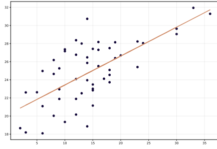
(a) Strengthening triangles corr = 0.67, p = 4.4 \times 10^{-8}
