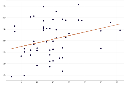
(c) Strengthening triangles corr = 0.31, p = 0.02
