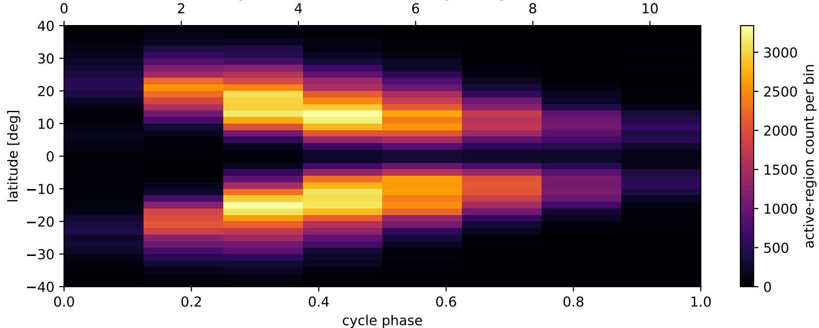
Average solar cycle: all 13 cycles folded together years since minimum (mean cycle length)
