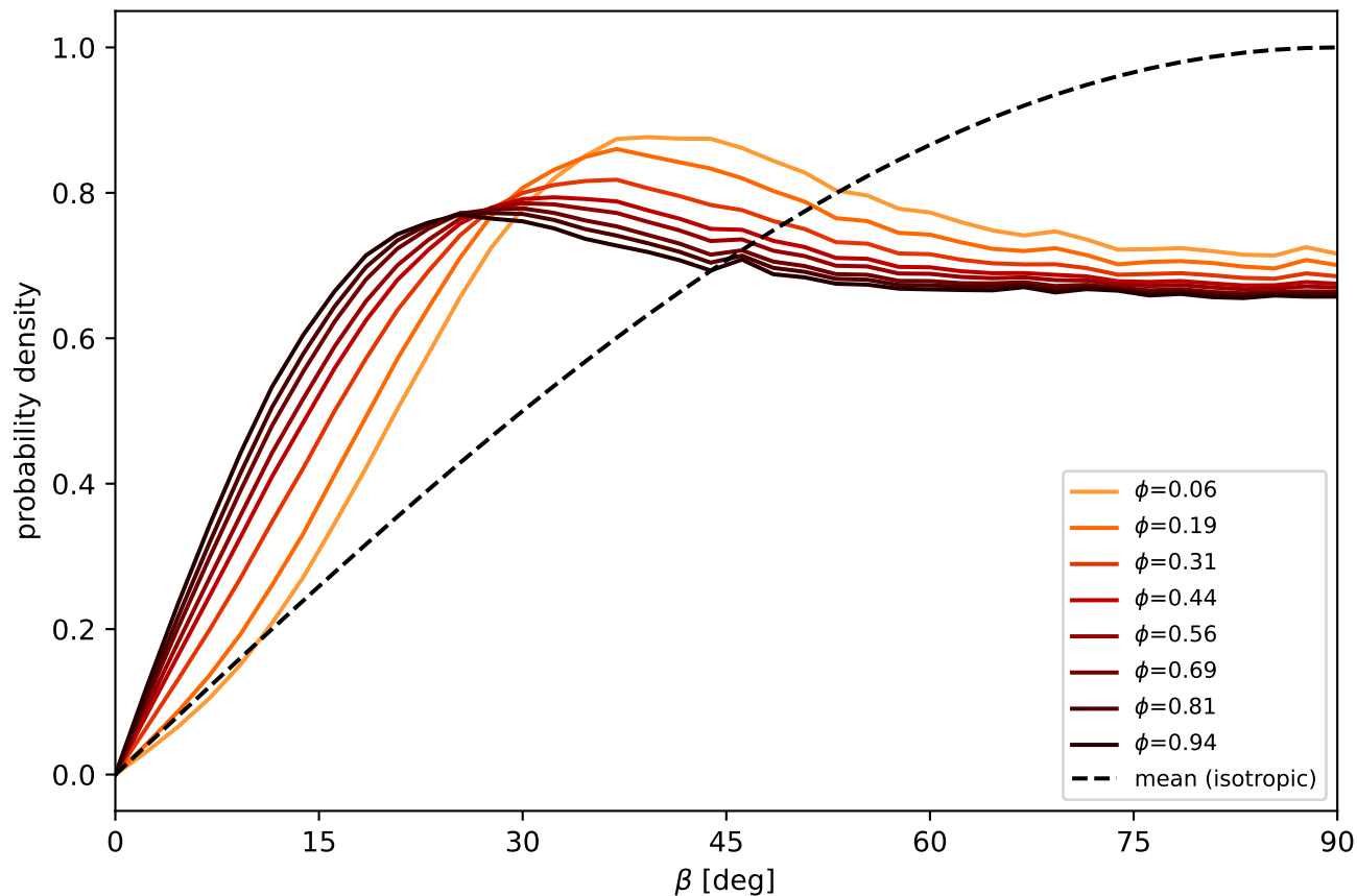
Sun ( \tau = 90^\circ ): CME viewing-angle distribution across the cycle
