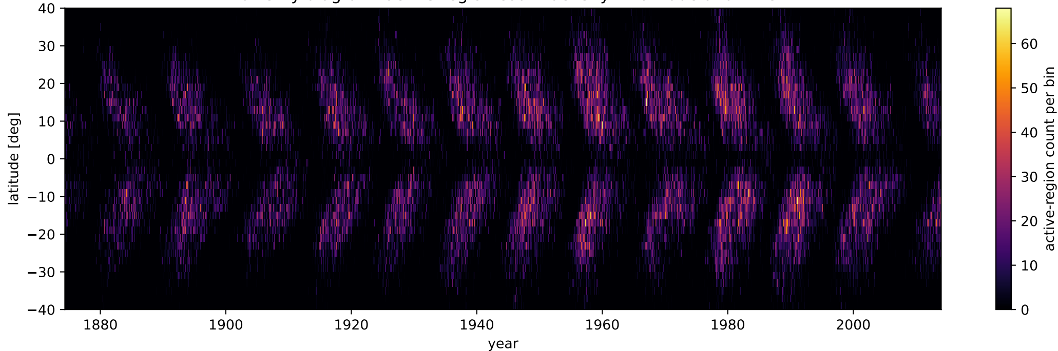
Butterfly diagram: active-region count density in latitude and time
