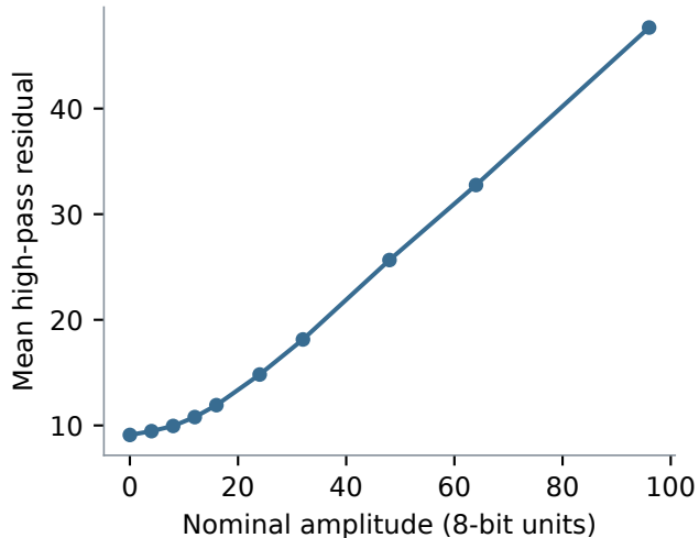
(a) Amplitude calibration
