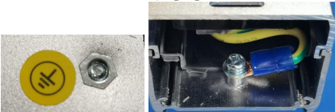
DMQY-TY10-XG20-KxXJqFUa2_Ut20_Ut65 接地
