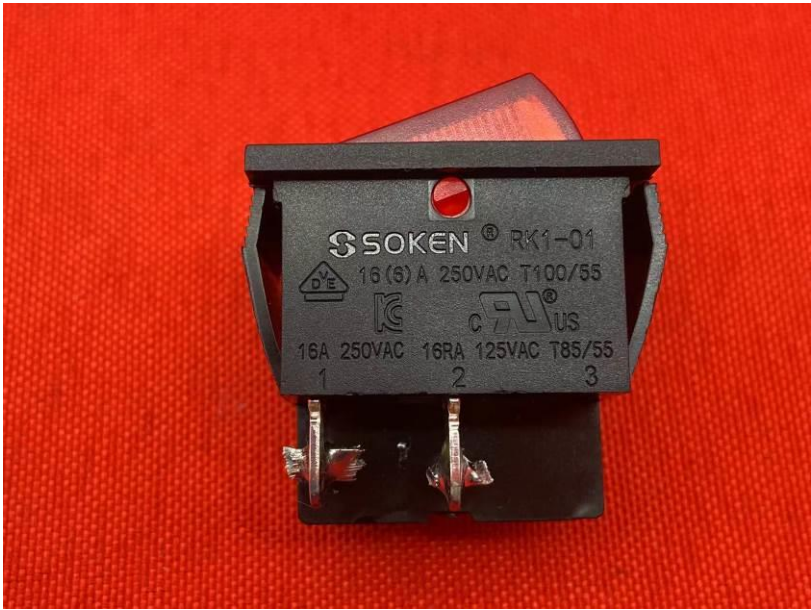
跷板开关 (RK1-01)
